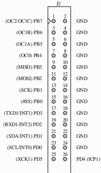
GU300 VFD Display (any display with suitable cable) Port B and Port pin PD0 - PD5
