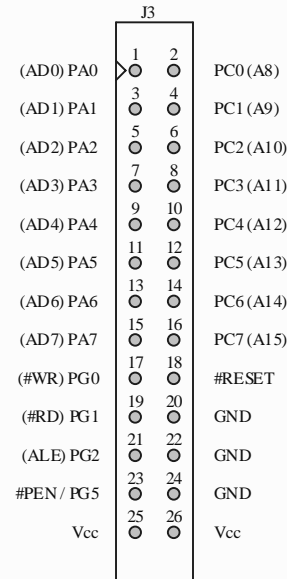
Memory Expansion Port A, Port C and Port G
